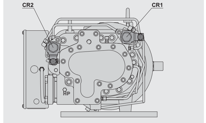
Fig. 5 Arrangement of solenoid valves
